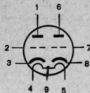
Noval B9A
